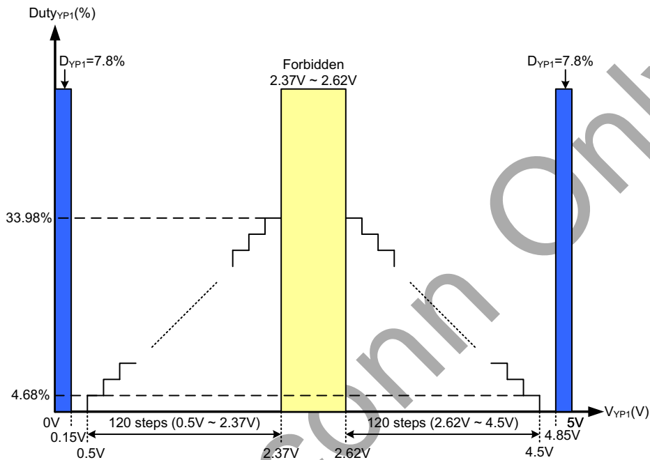
Figure : YP1 Voltage Setting Range
