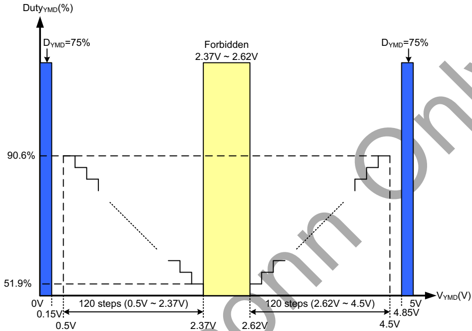
Figure : YMD Voltage Setting Range
