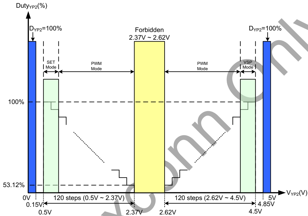
Figure : YP2 Voltage Setting Range
