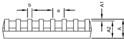
TSSOP-16 (FD) Package
